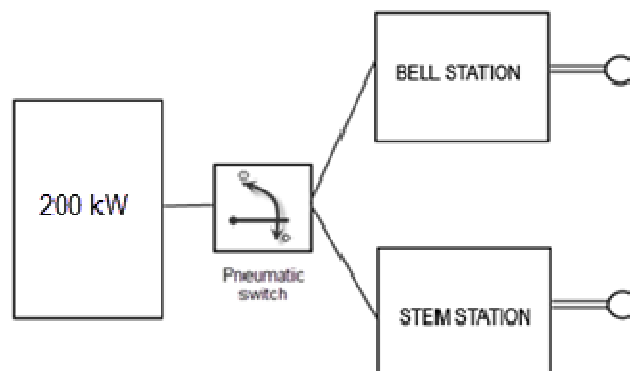
Fig.19 Oscillating circuit scheme including with its switched power.
