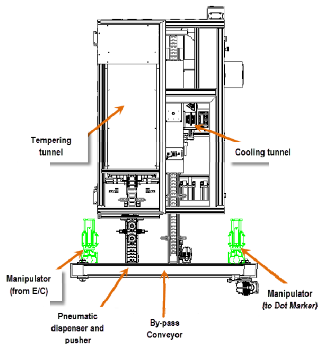
Fig.13 Tempering tunnel diagram.
