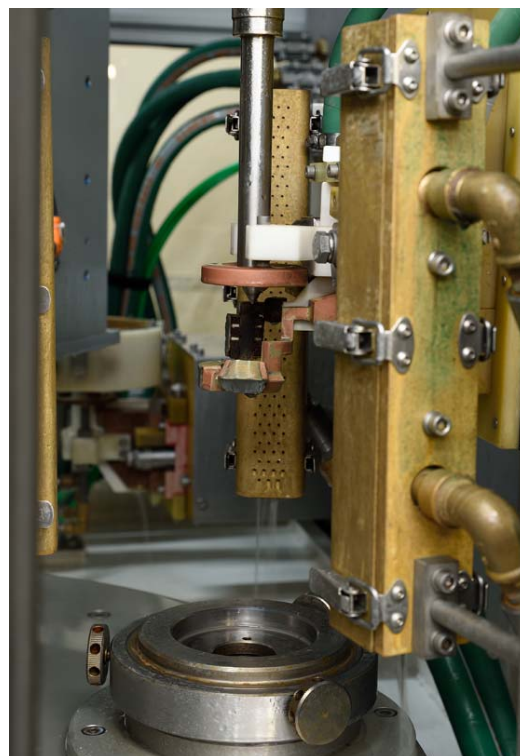
Fig. 21: Stem single-shot coil and quench set
