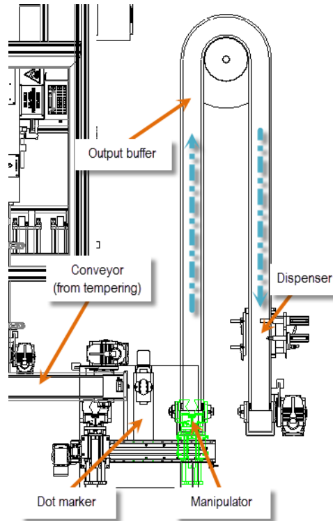
Fig.17 Dot marking and output buffer diagram.
