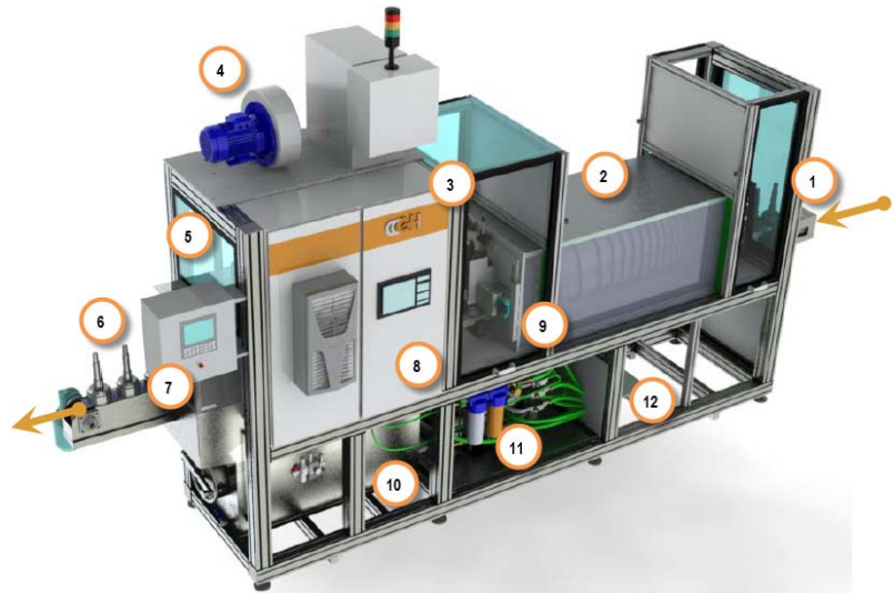
Fig.15 Tempering coil and composite conveyor.
