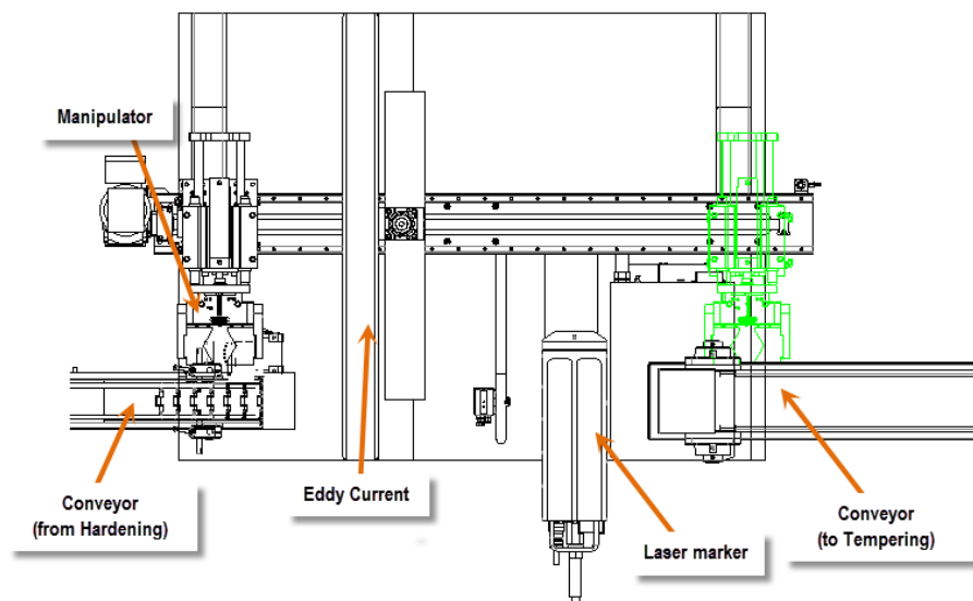
Fig.12 Eddy current and laser station.
