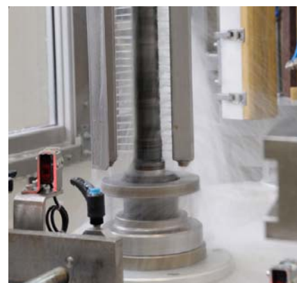
Fig.10 Auxiliary quench.
