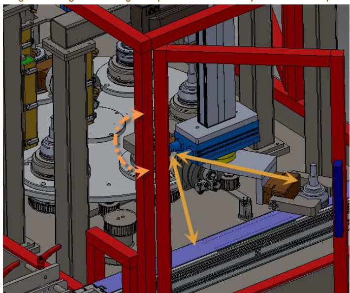
Fig.5 Loading and turning manipulator with double pneumatic clamps.
